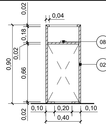
DET.01 - CUBA VERTICAL
