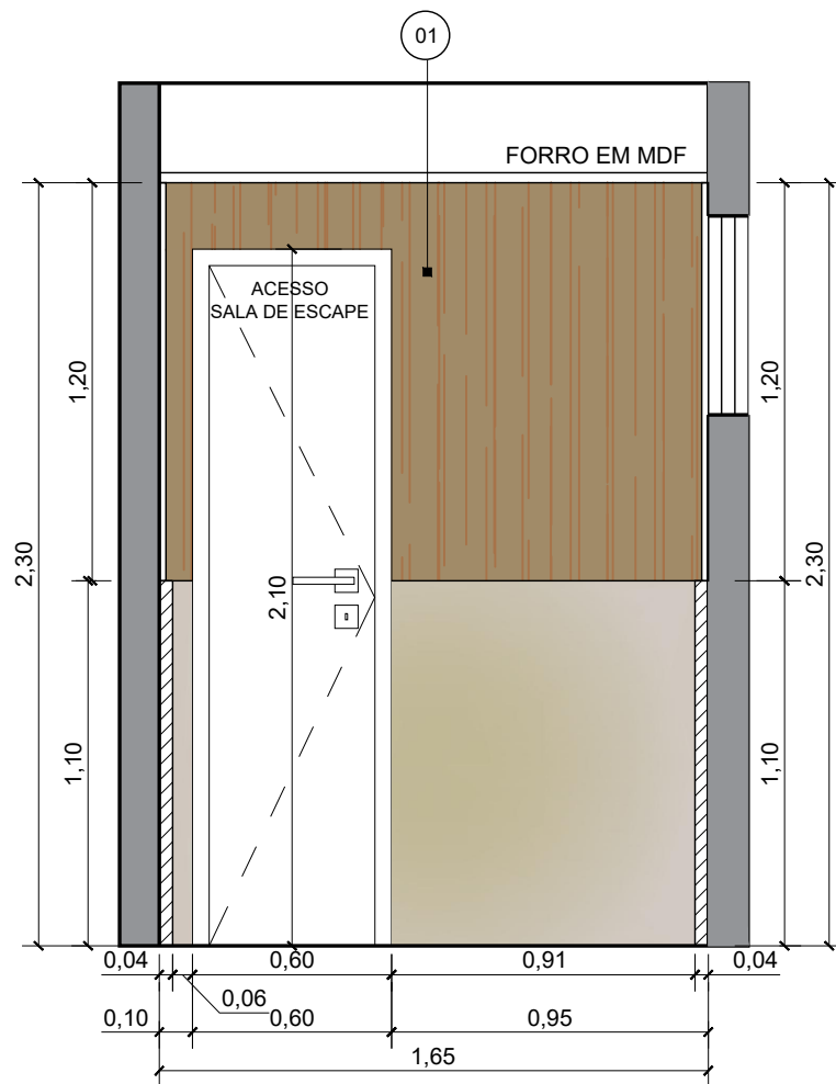
VISTA C - BAN. SOCIAL
