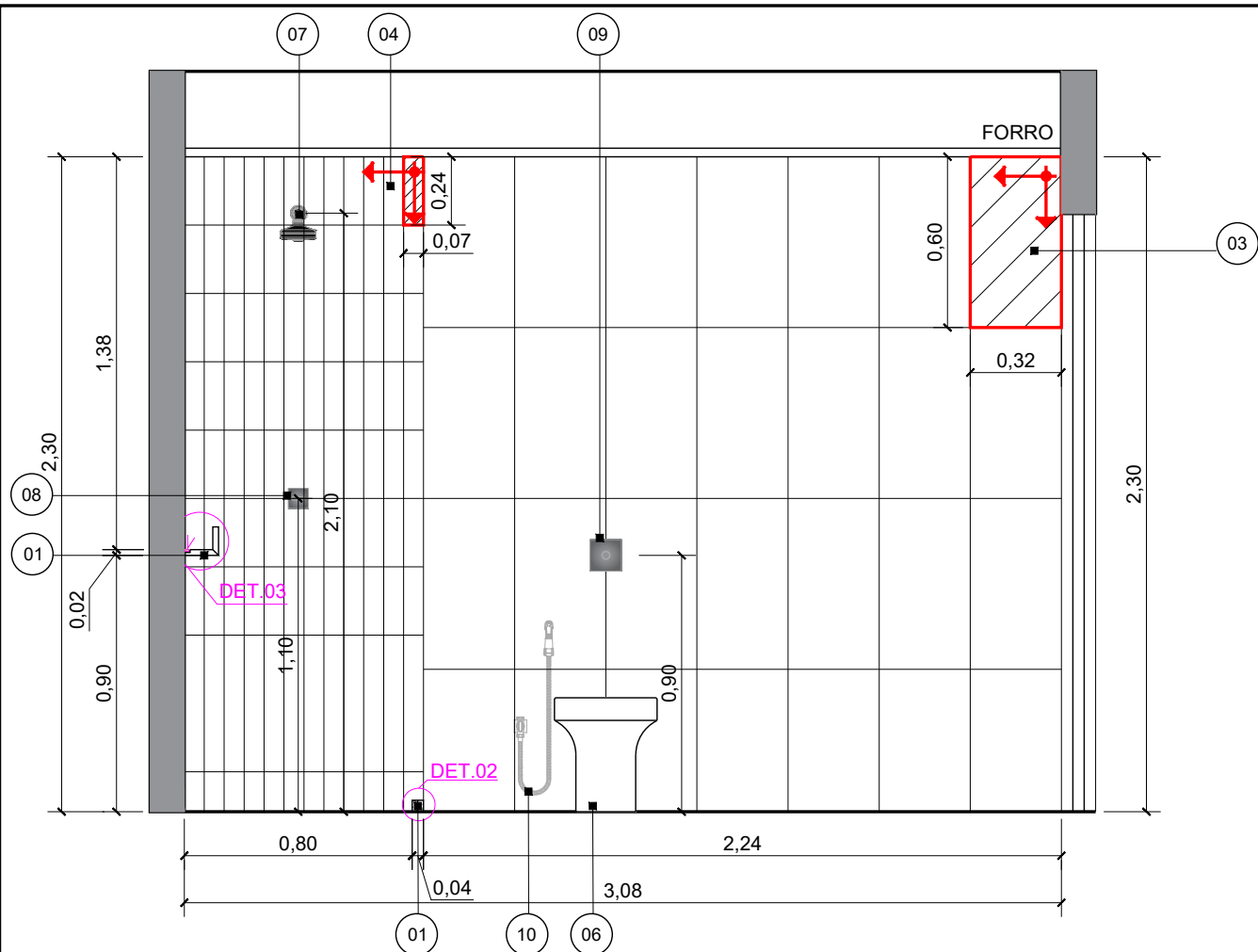
VISTA C - BAN. SOCIAL
