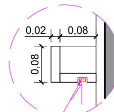
DET.08 - LED PRATELEIRA
